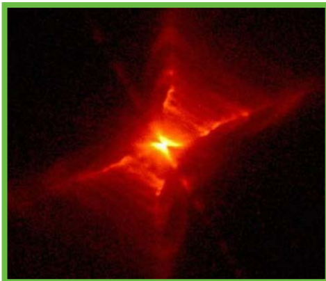
Red Rectangle Nebula
